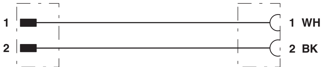
Circuit diagram
