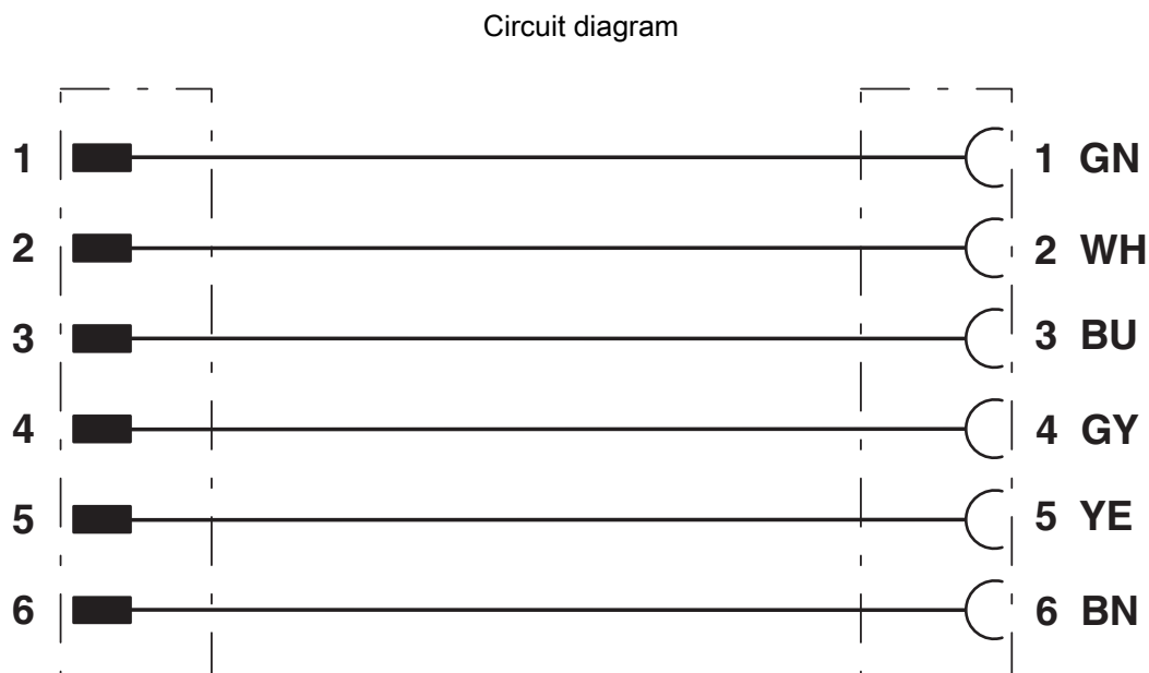
Contact assignment of 7/8" plugs/sockets
