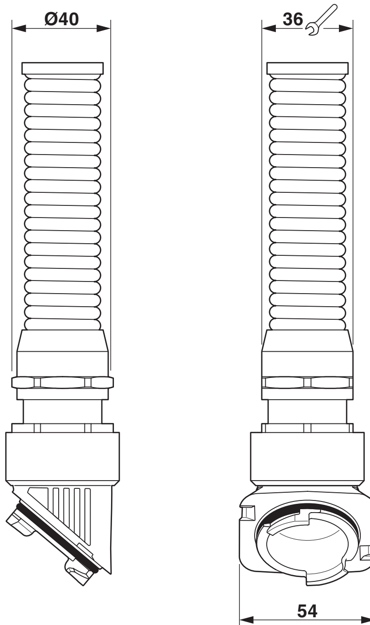
Dimensional drawing
