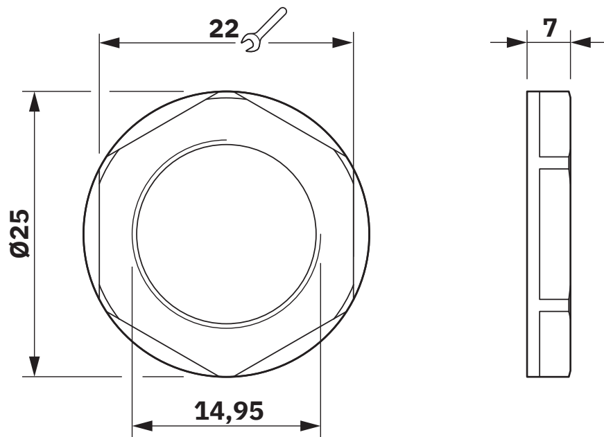
Dimensional drawing
