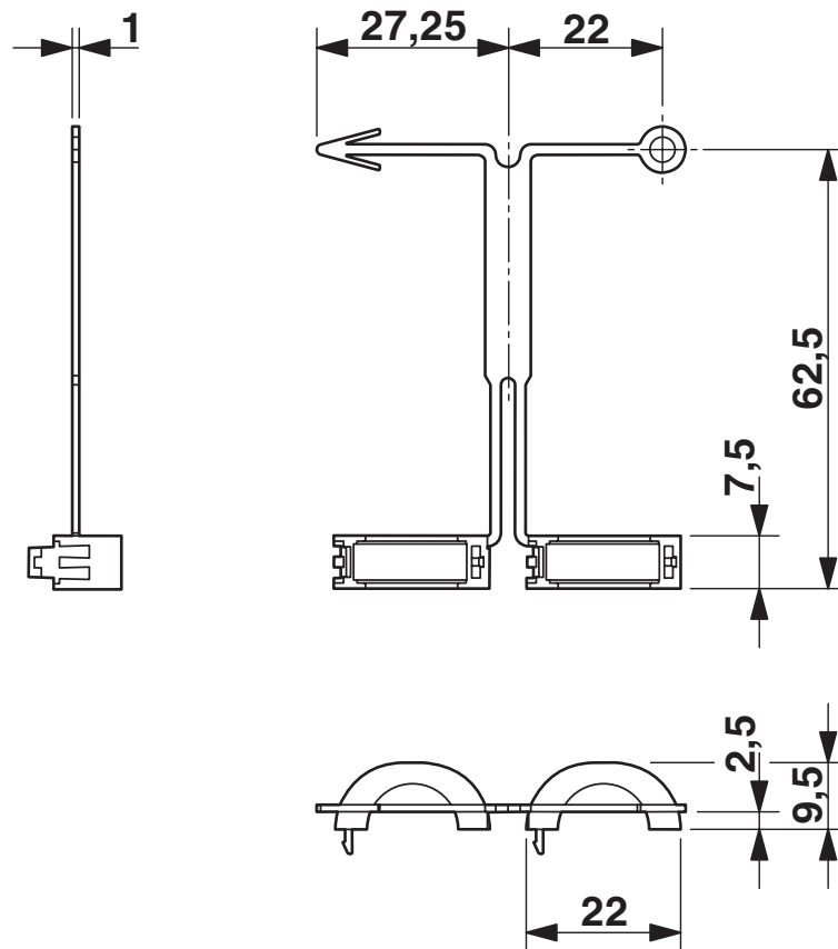
Dimensional drawing
