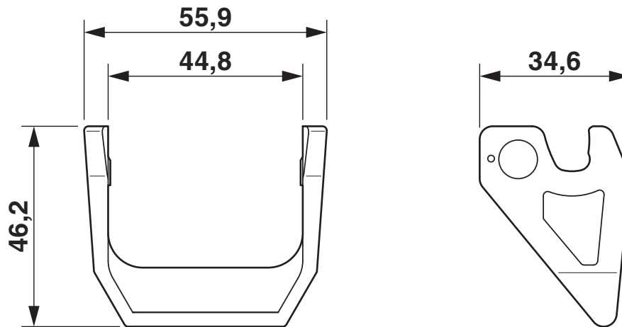
Dimensional drawing
