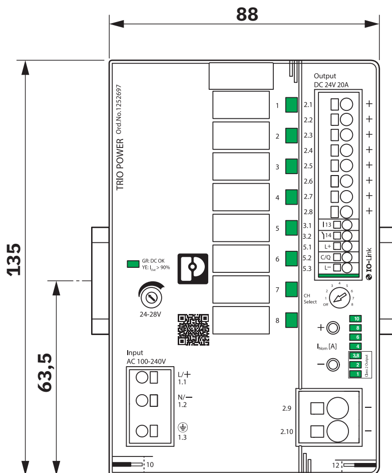
Dimensional drawing
