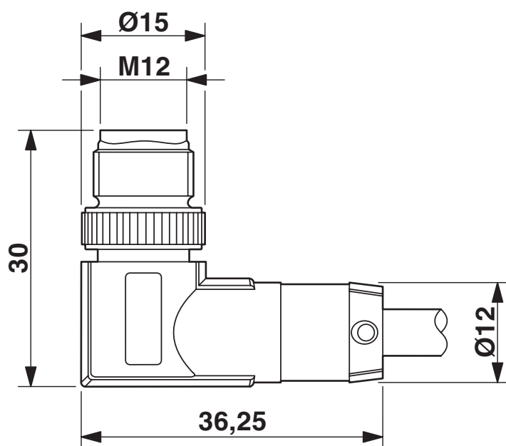
Dimensional drawing
