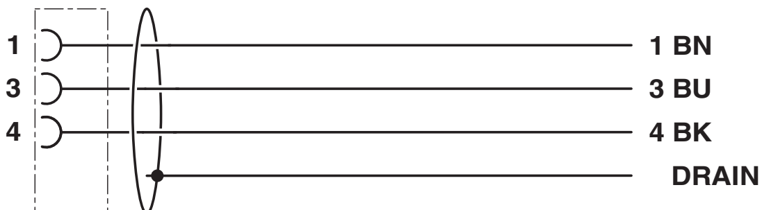
Contact assignment of the M12 socket
