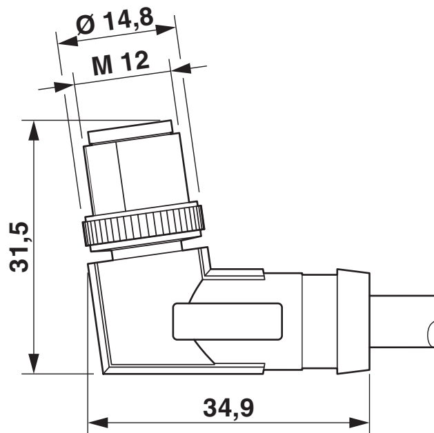
Dimensional drawing
