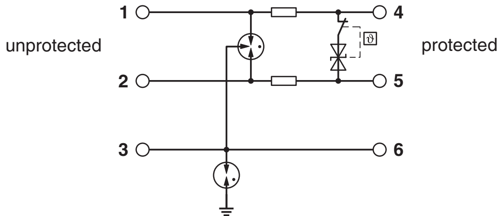
Circuit diagram
