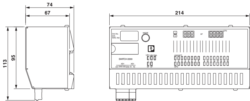
Dimensional drawing
