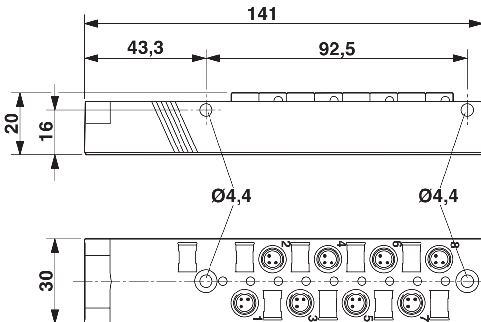
Dimensional drawing
