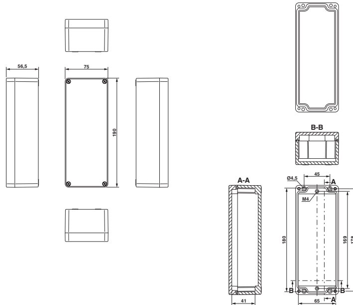
Dimensional drawing
