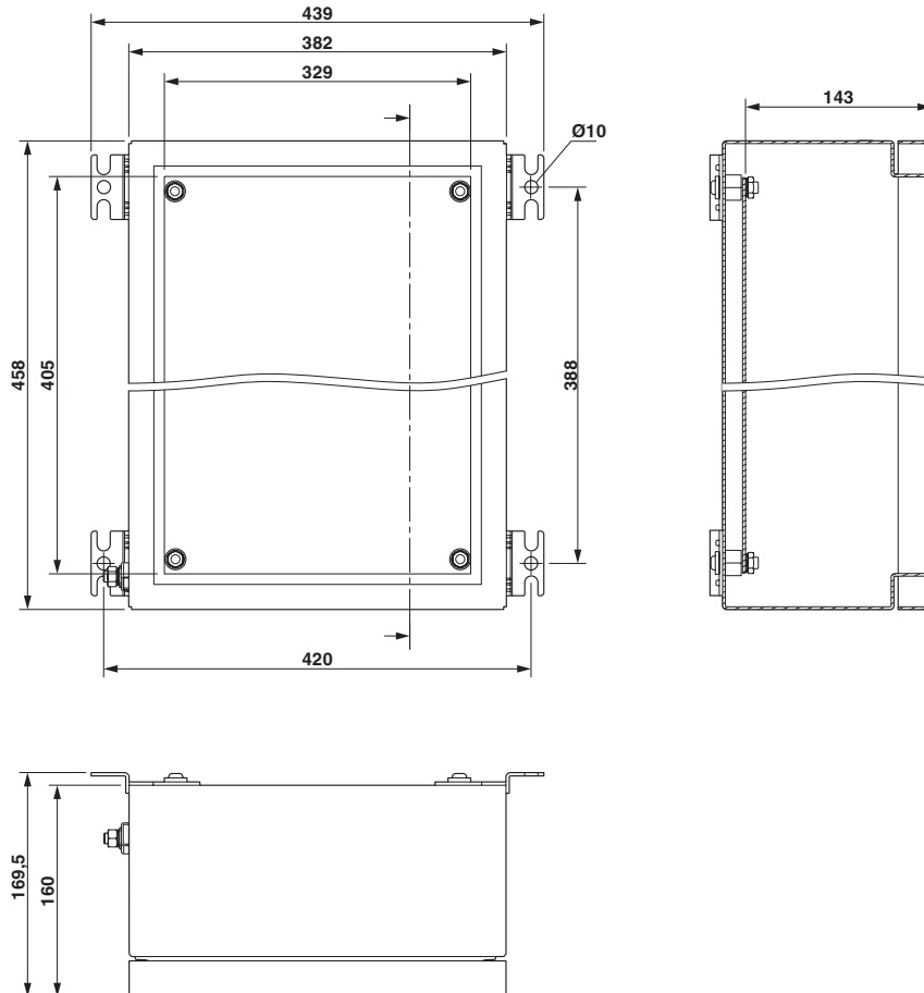
Dimensional drawing
