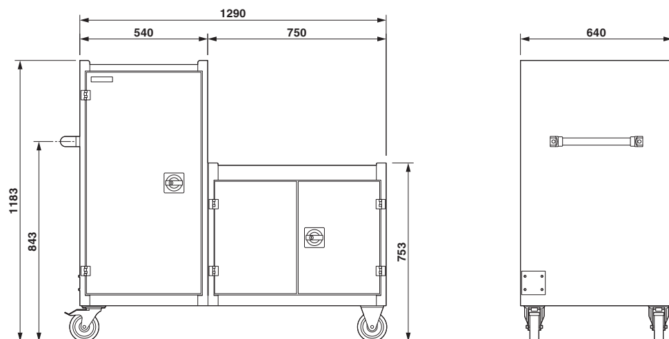
Dimensional drawing
