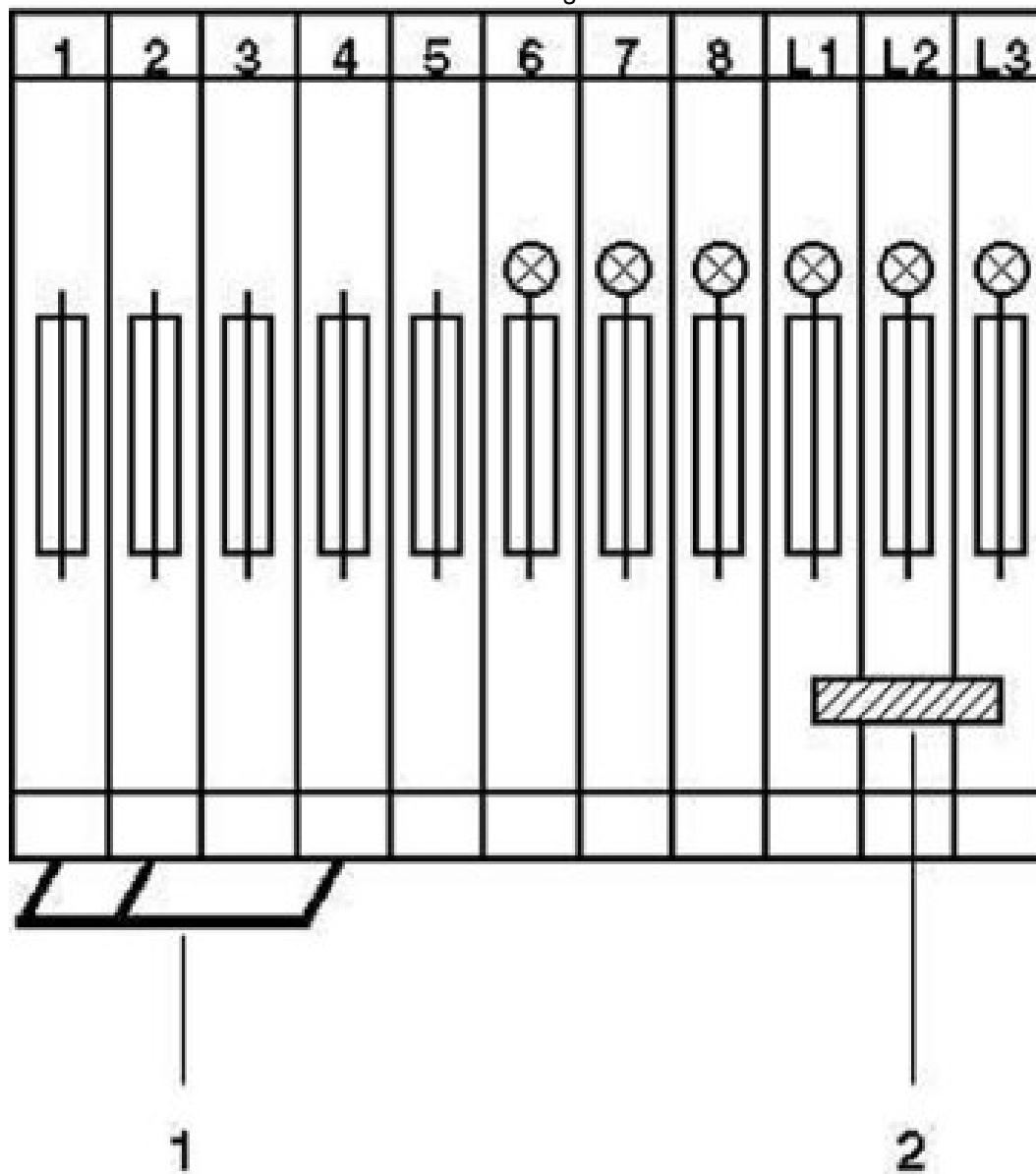
Circuit diagram
