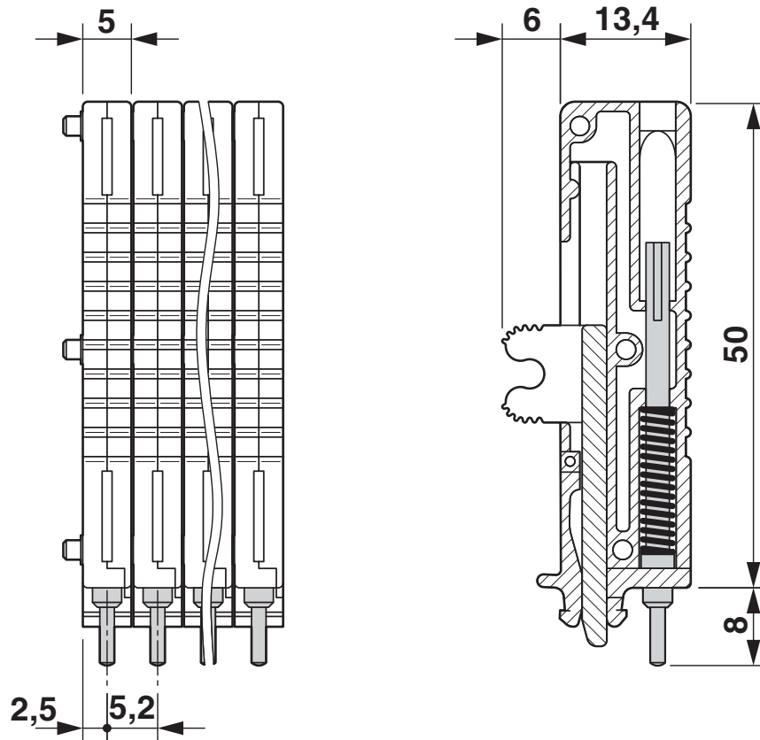
Dimensional drawing
