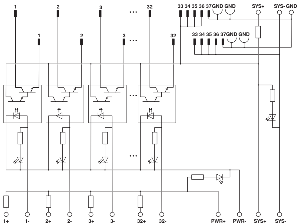
Circuit diagram
