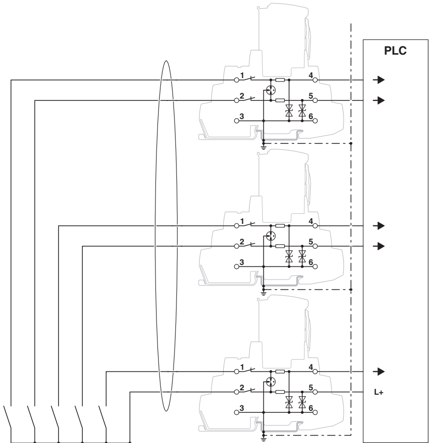
Application drawing
