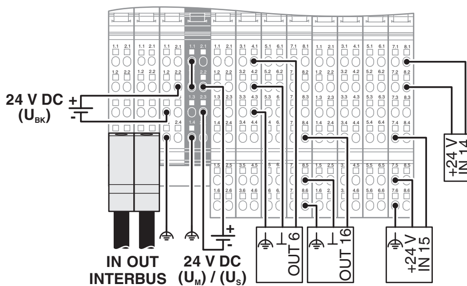
Connection diagram
