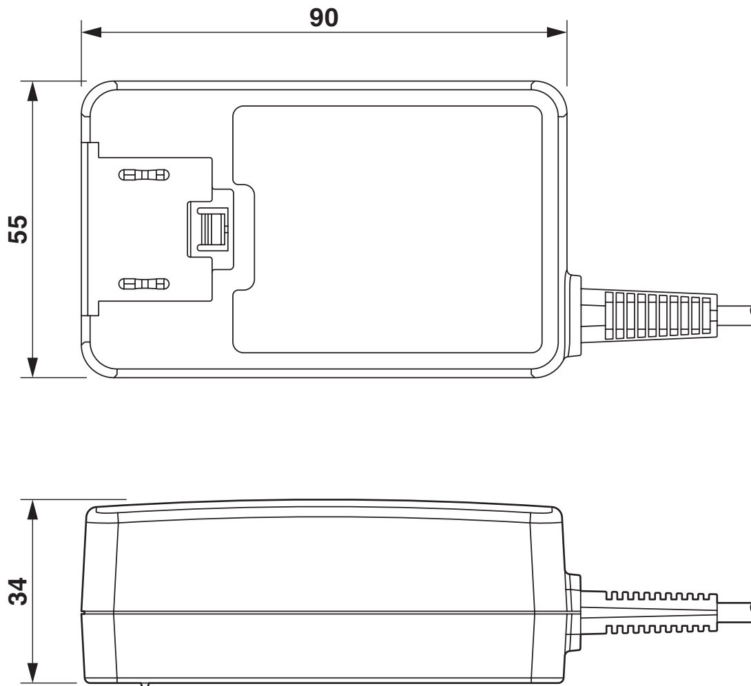
Dimensional drawing
