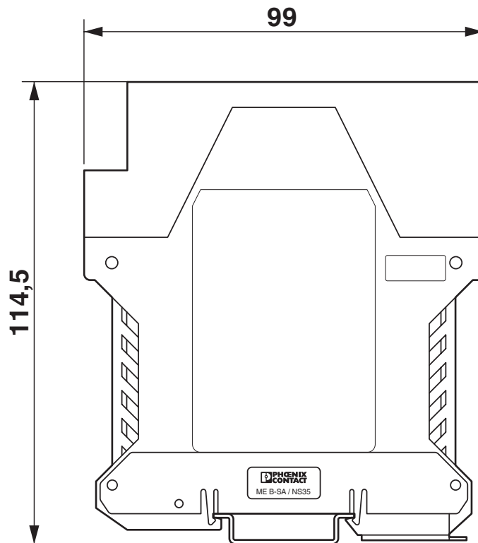
Dimensional drawing
