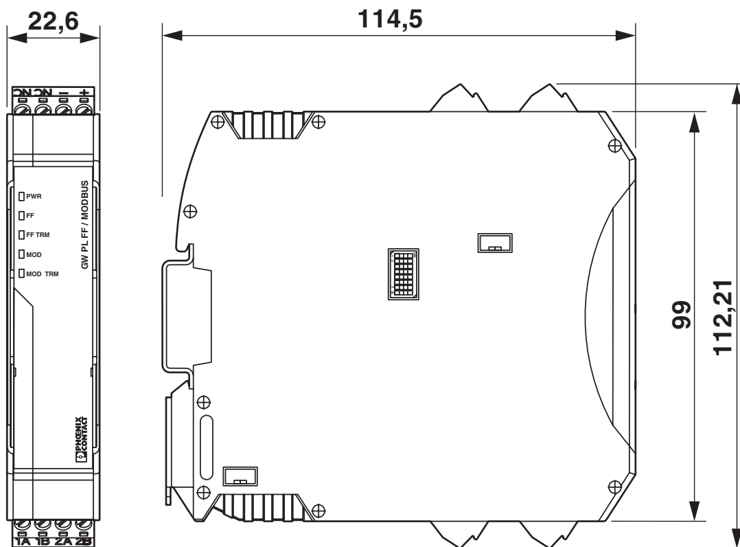
Dimensional drawing
