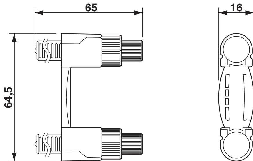
Dimensional drawing
