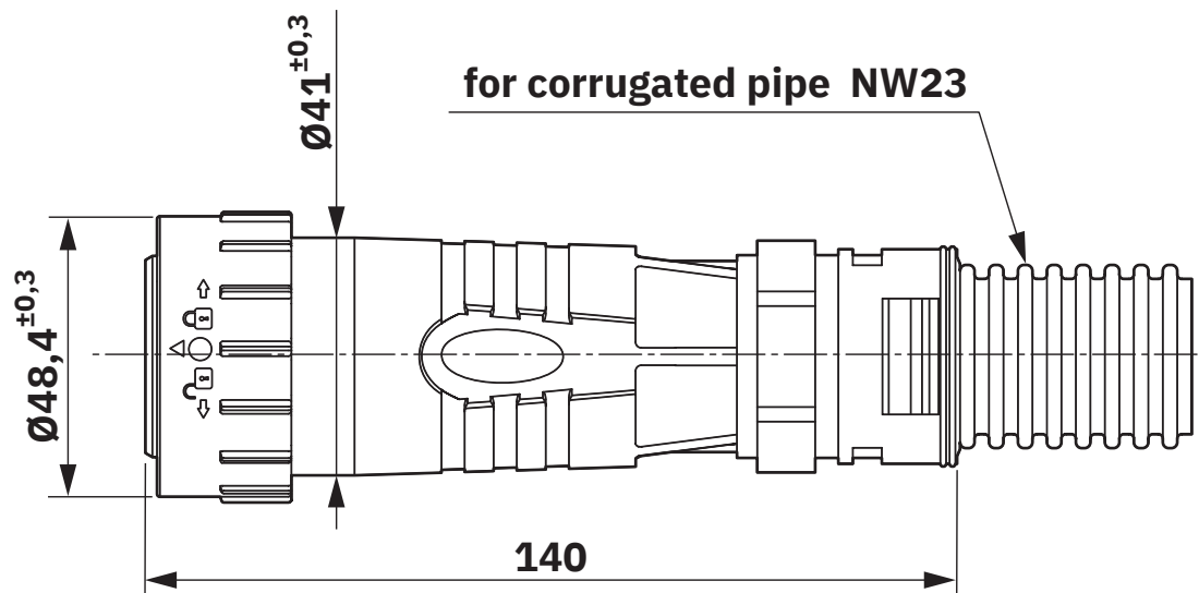
AHDP06-24-91S-BS3 connector with conduit adapter NW23
