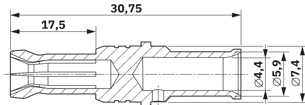
Dimensional drawing
