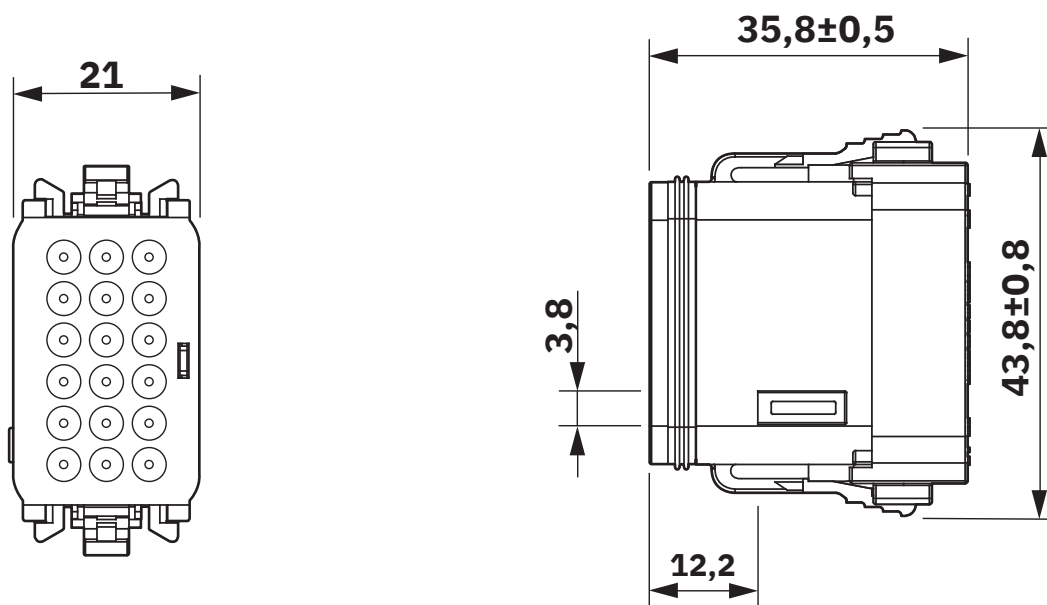
AT16-18SA top view and side view
