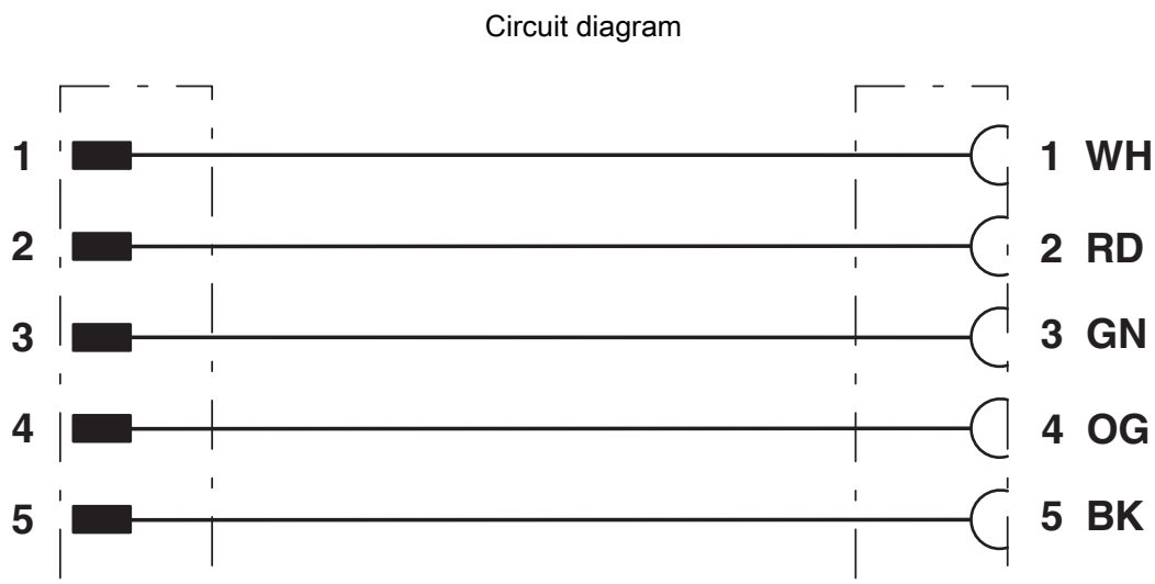
Contact assignment of 7/8" plugs/sockets
