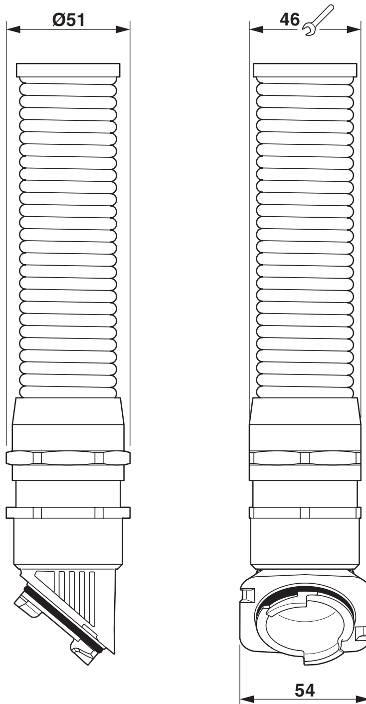
Dimensional drawing
