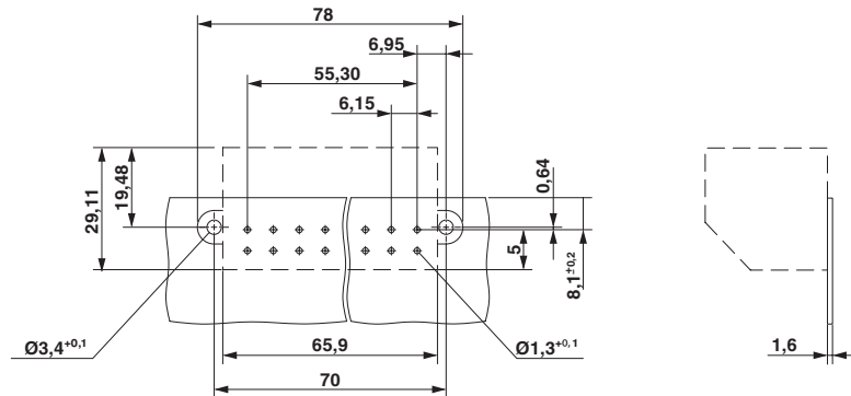
Dimensional drawing
