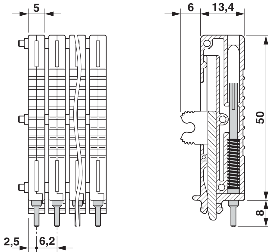
Dimensional drawing
