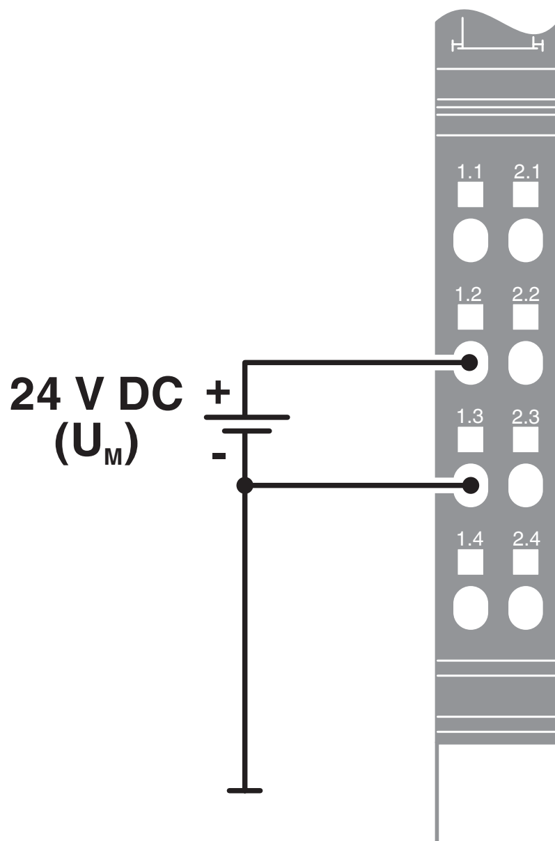
Connection diagram
