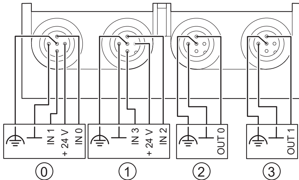
Connection diagram
