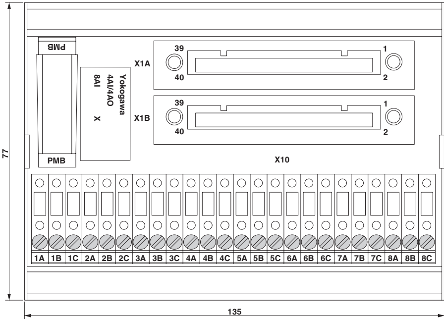
Dimensional drawing
