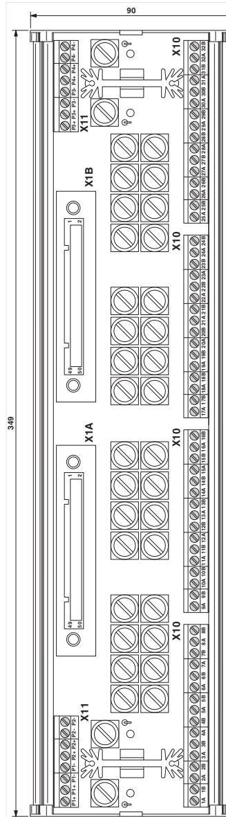
Dimensional drawing
