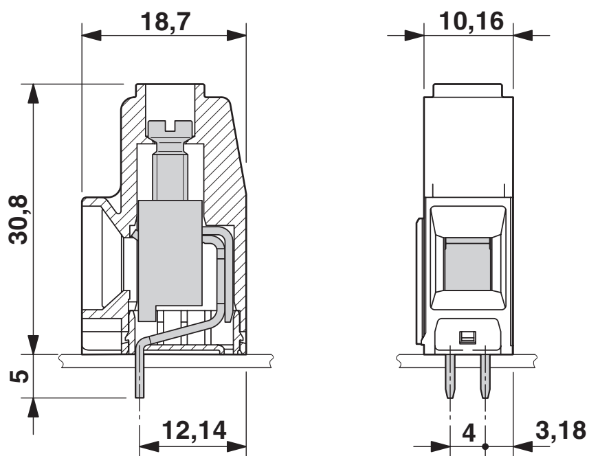
Dimensional drawing
