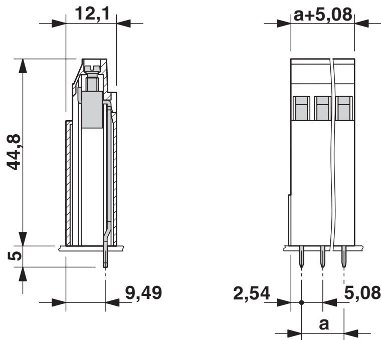
Dimensional drawing
