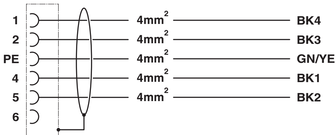
Circuit diagram
