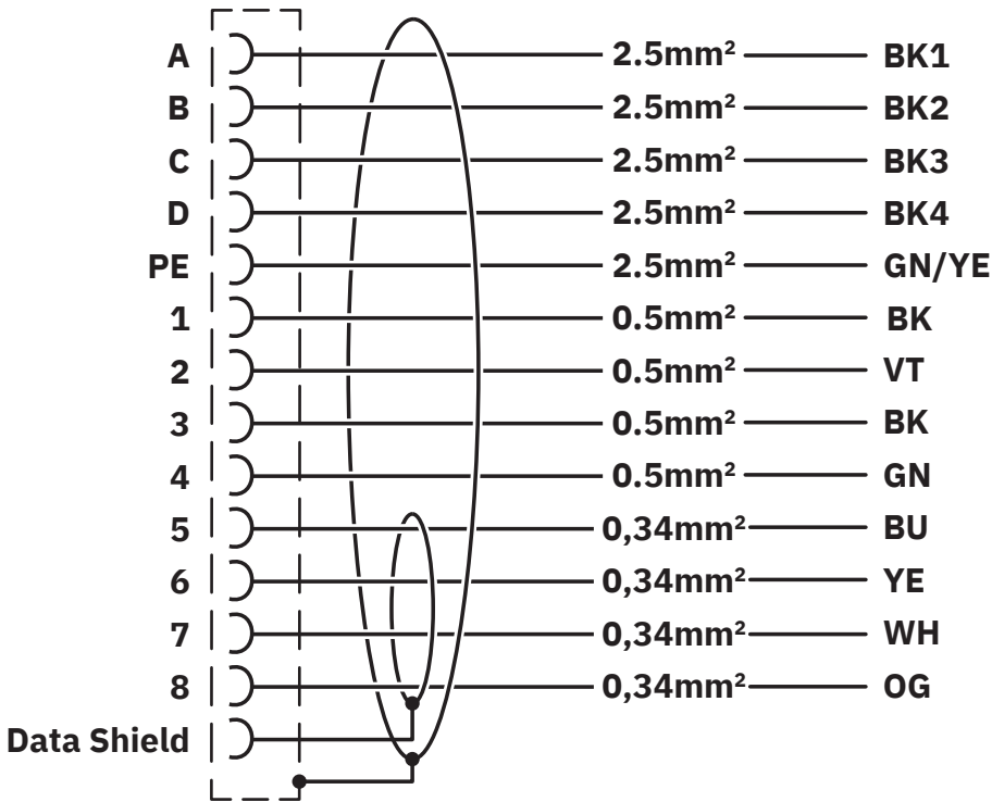
Circuit diagram
