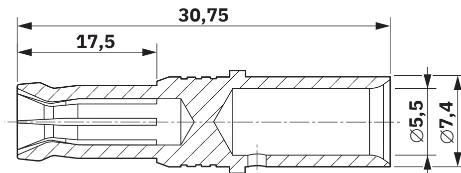
Dimensional drawing
