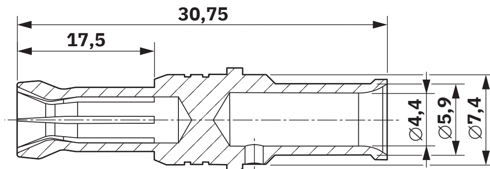
Dimensional drawing
