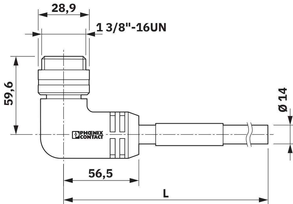
Dimensional drawing
