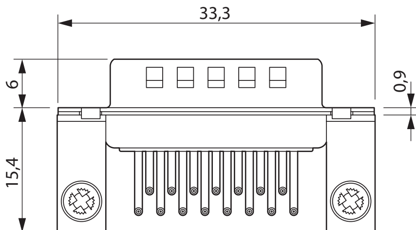
Dimensional drawing
