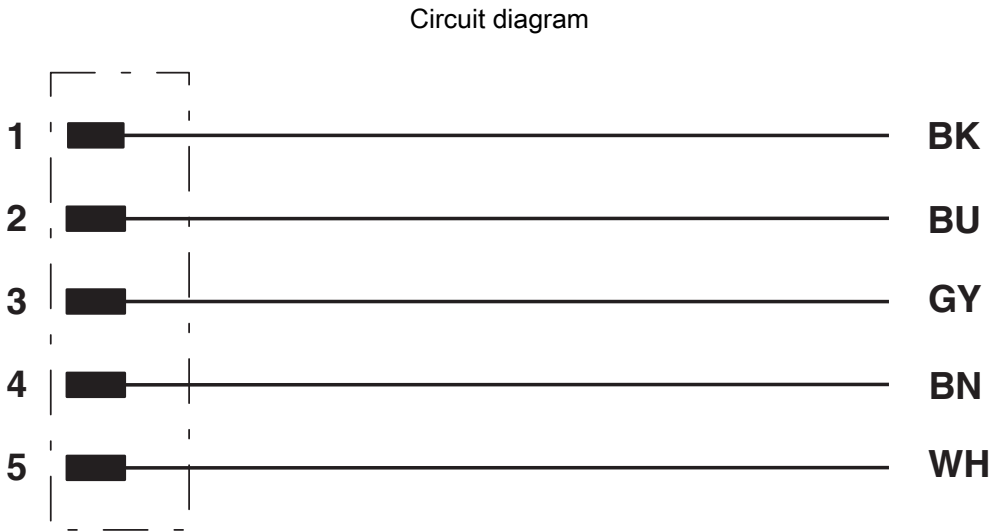
Contact assignment of 7/8" plug
