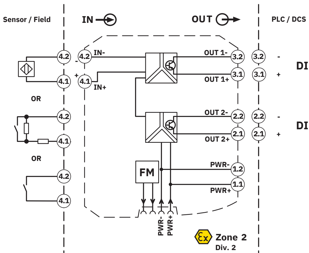
Block diagram
