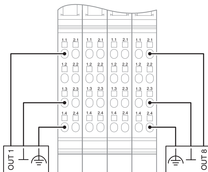
Connection diagram
