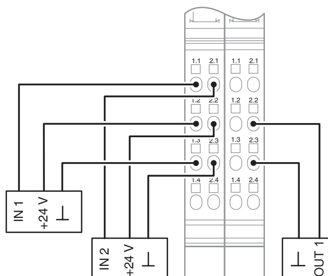
Connection diagram
