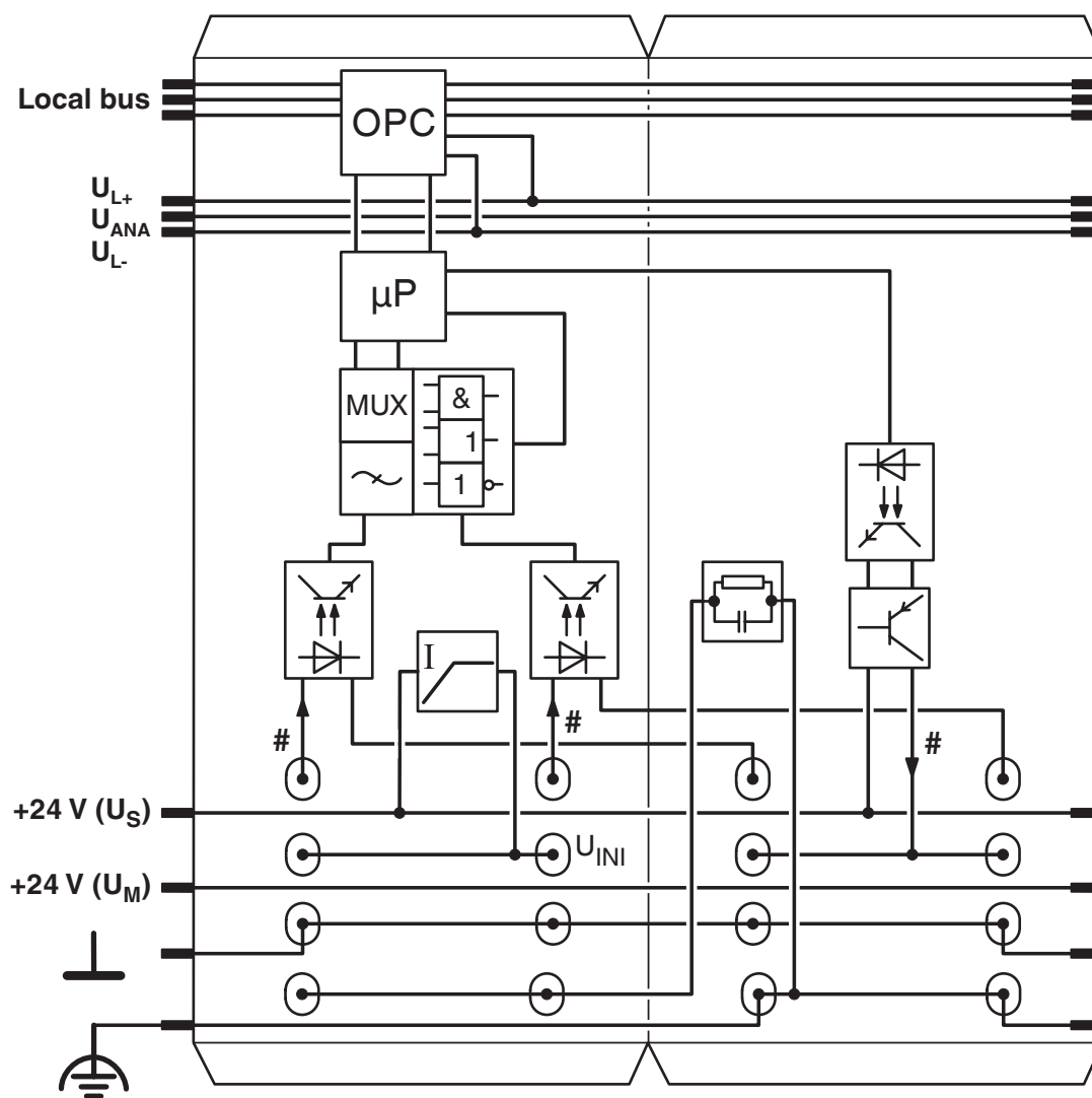
Block diagram
