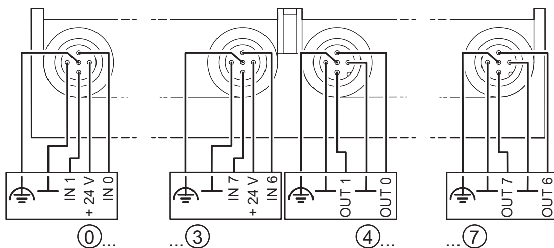
Connection diagram
