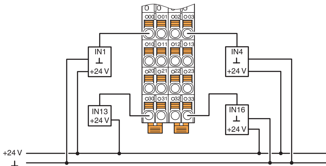
Connection in 1-conductor technology
